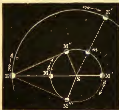
FIG. 13.—Orbit of Mercury and Earth.
